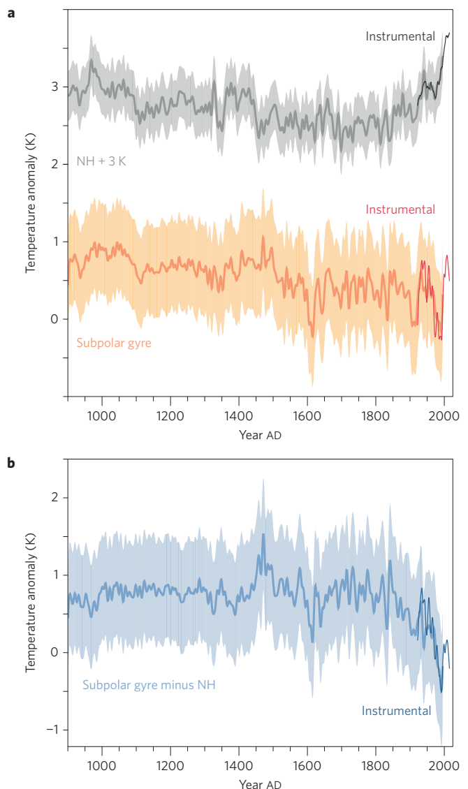
Figure 3 | Surface temperature time series for different regions. Data from the proxy reconstructions of Mann et al. 12,13 , including estimated 2- \sigma uncertainty bands, and from the HadCRUT4 instrumental data 49 . The latter are shown in darker colours and from 1922 onwards, as from this time on data from more than half of all subpolar-gyre grid cells exist in every month (except for a few months during World War II). The orange/red curves are averaged over the subpolar gyre, as indicated on Fig. 1. The grey/black curves are averaged over the Northern Hemisphere, offset by 3 K to avoid overlap. The blue curves in the bottom panel show our AMOC index, namely the difference between subpolar gyre and Northern Hemisphere temperature anomalies (that is, orange/red curves minus grey/black curves). Proxy and instrumental data are decadal smoothed.
